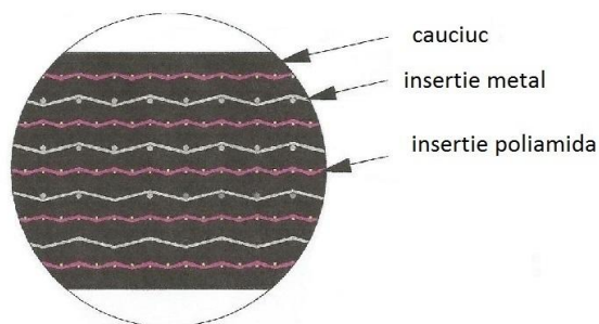
DETALIU " D "
